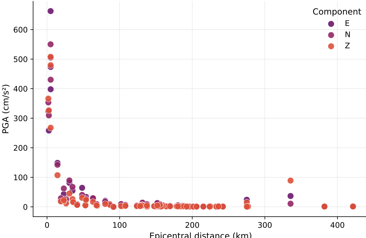
PGA vs epicentral distance by component
